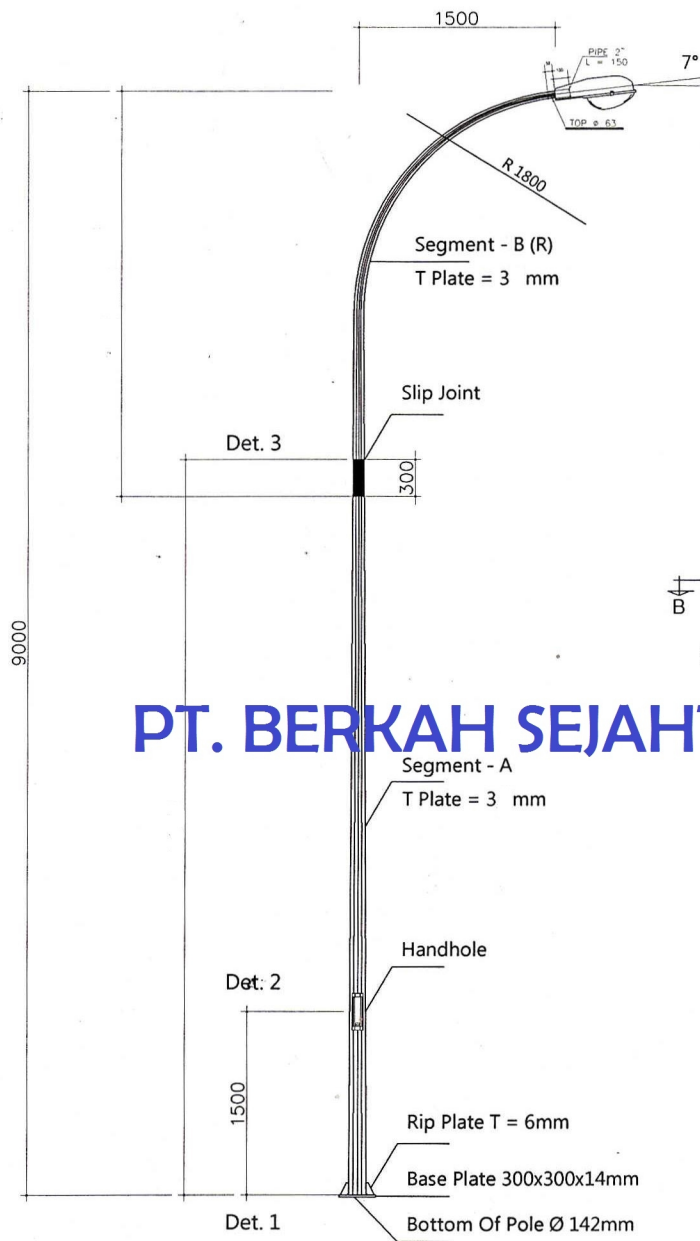
TIANG PJU H-09M SINGLE PARABOLE SCALE 1 : 25
